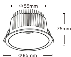
7-10W
