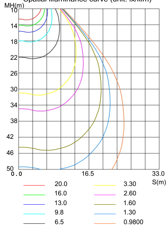
Spatial illuminance curve (unit: lx/klm)
